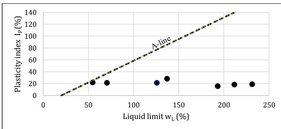
Figure 4: Casagrande plasticity chart for organic diatomite (with A-line).
